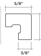
QUARTER SQUARE COVE 5/8" X 5 3/4" DISC01
